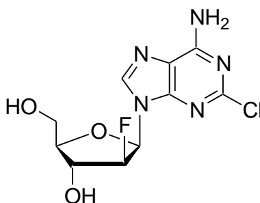
Clofarabine
